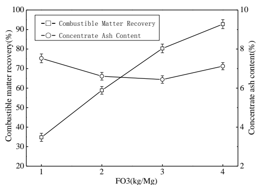
Fig. 7. Flotation results at different collector dosage of FO3
